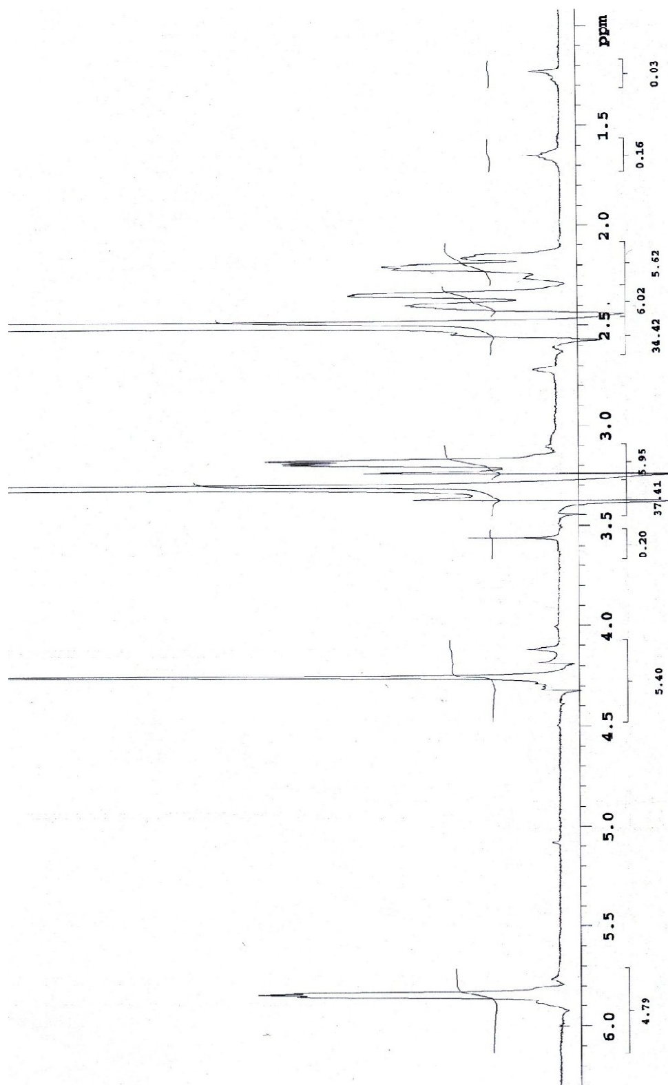
Figure 3.15: 1 H-NMR of (AM-6).
